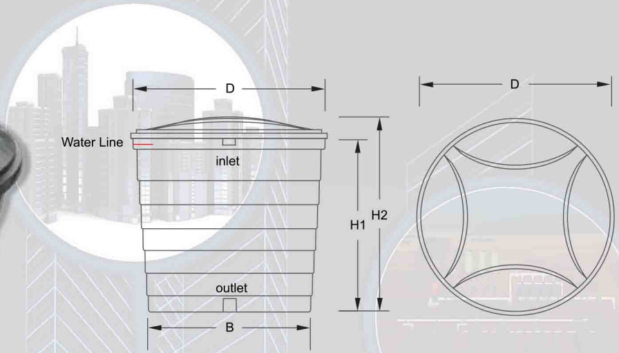
PE COLD WATER STORAGE TANK (ROUND) DIMENSION
